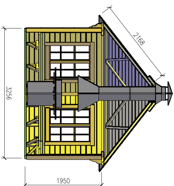
CUT VIEW
